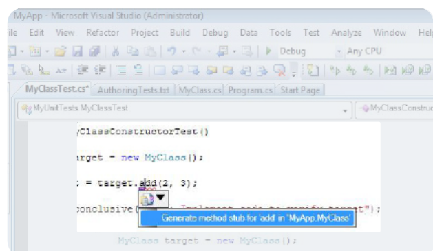
TEST DRIVEN DEVELOPMENT- CONSUME FIRST, DECLARE SECOND
